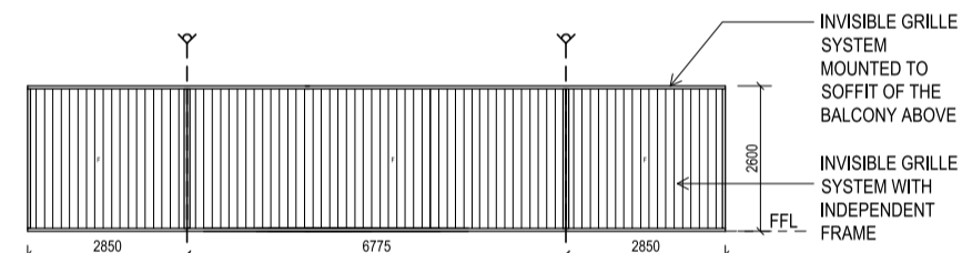
BALCONY SCREEN ELEVATIONS (TYPE A) (EVEN FLOORS)
