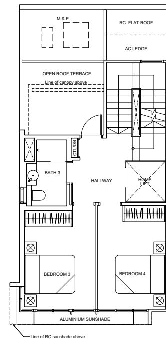
ATTIC
