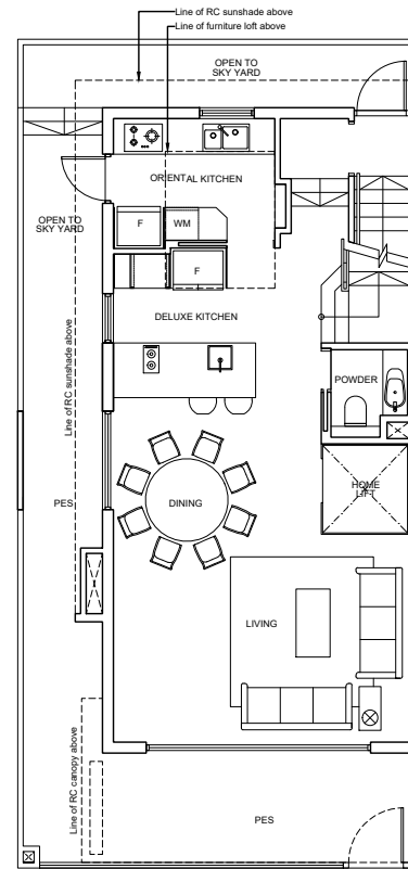
1ST STOREY
