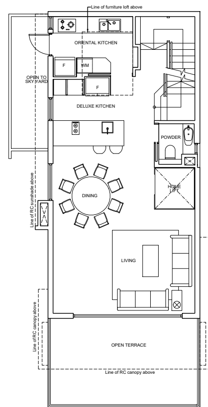
2ND STOREY
