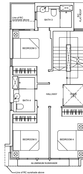
3RD STOREY
