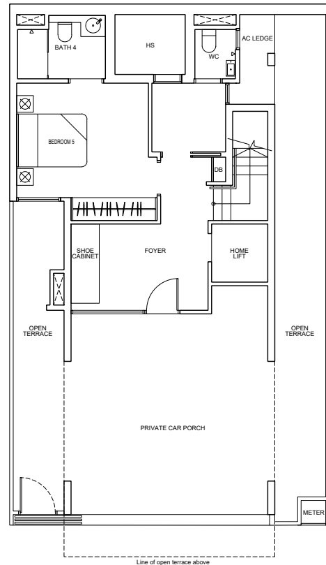
1ST STOREY
