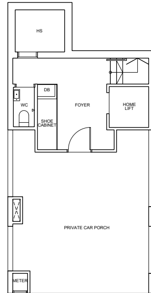
BASEMENT
