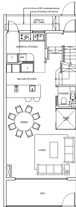
1ST STOREY
