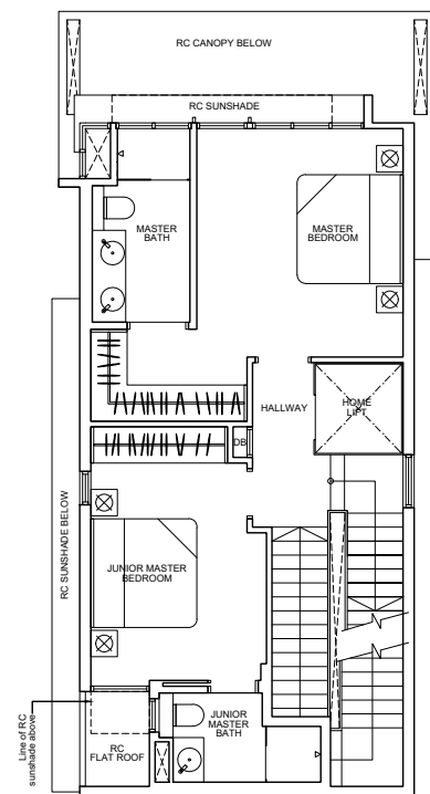
2ND STOREY
