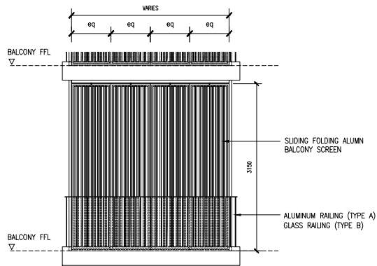
TYPICAL BALCONY SCREEN - ELEVATION 1
