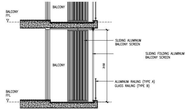
TYPICAL BALCONY SCREEN - SECTION A - A
