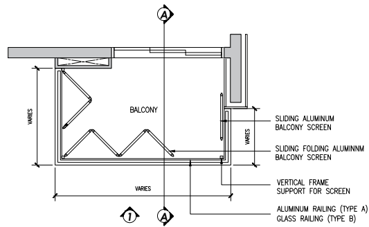
TYPICAL BALCONY SCREEN - PLAN
