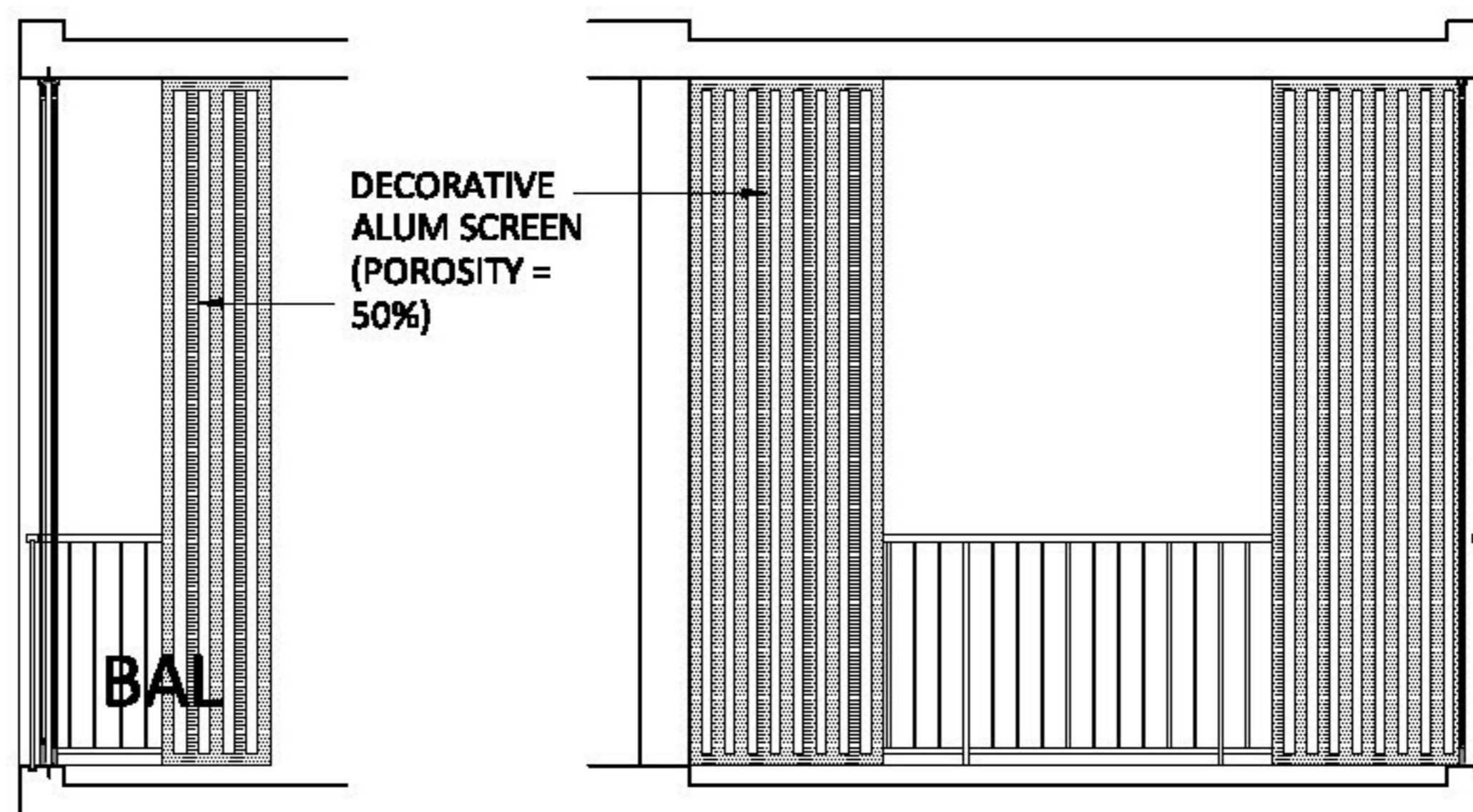
SECTION X1-X1 (SCREEN OPEN)
