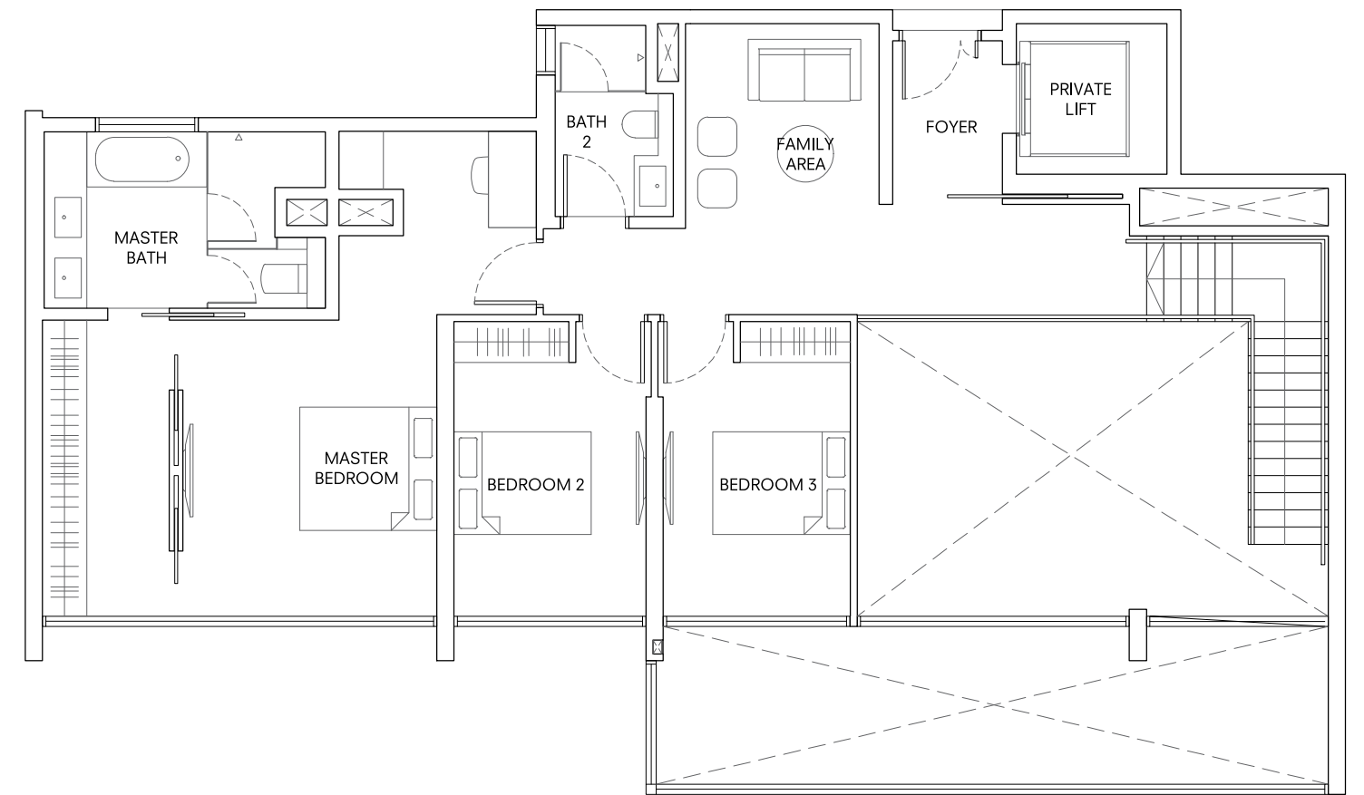
UPPER FLOOR
