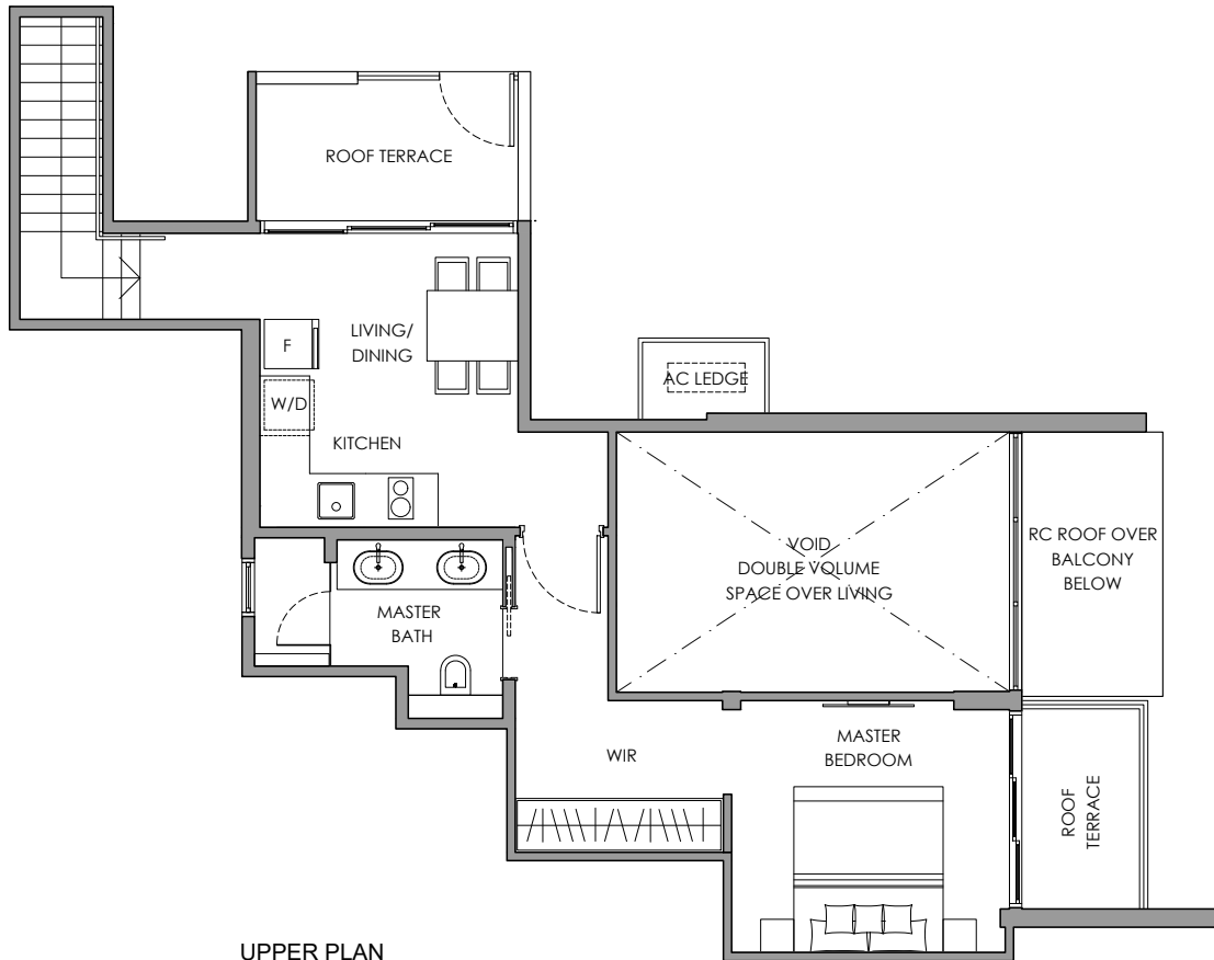
UPPER PLAN
