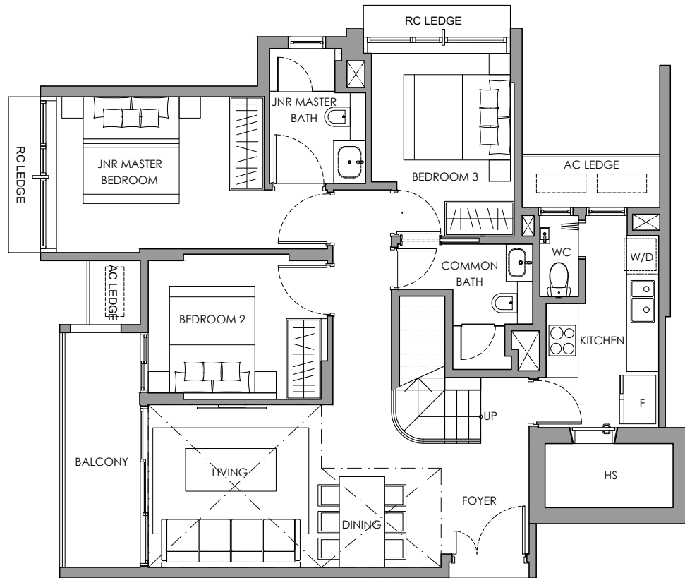
LOWER PLAN
