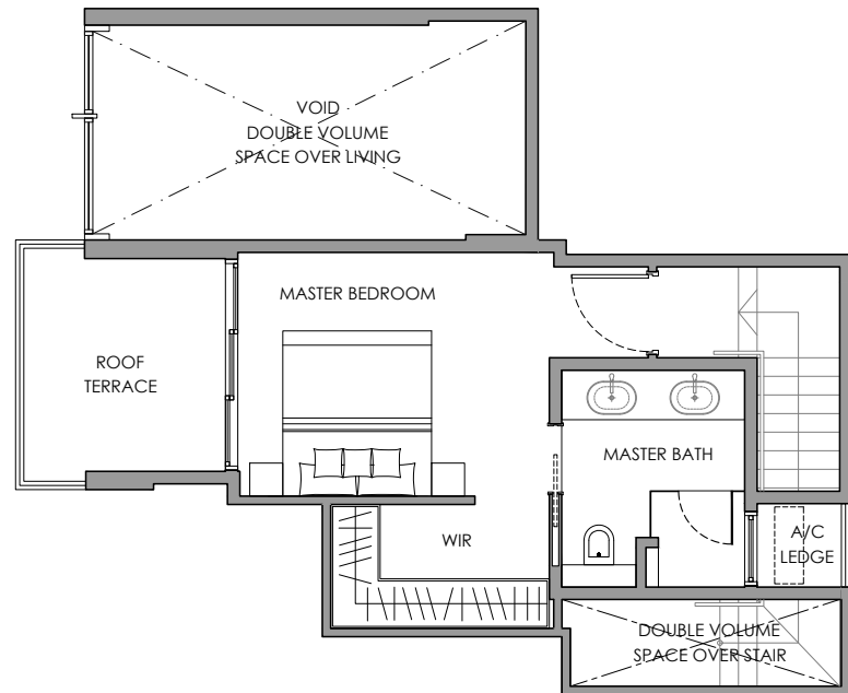
UPPER PLAN
