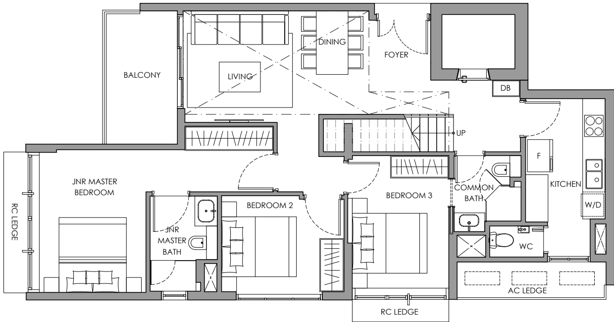
LOWER PLAN
